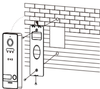
Wall bracket mounting
